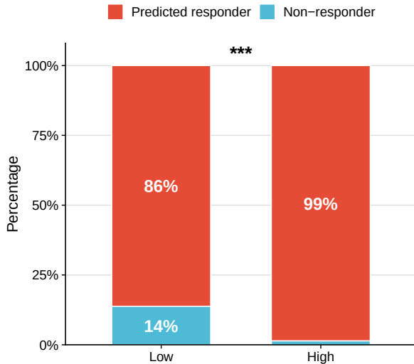
KIRP TIDE-predicted response
